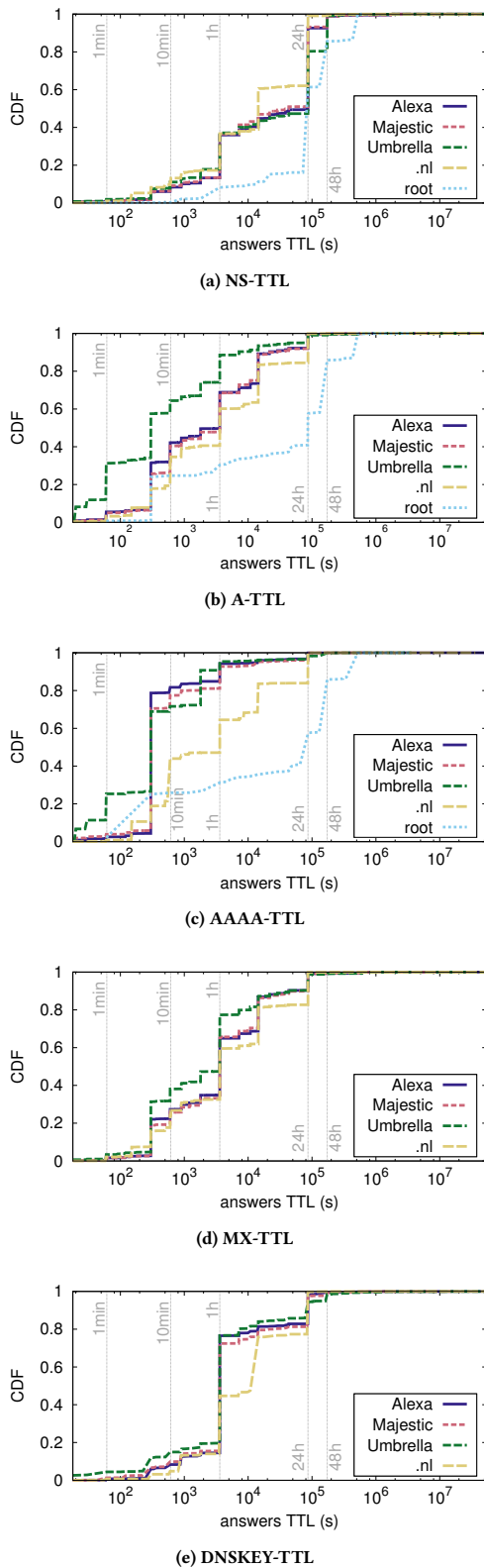
Figure 9: CDF of TTLs per record type, for each list.
