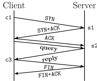
Fig. 1. TCP Handshake and RTT Measurements
